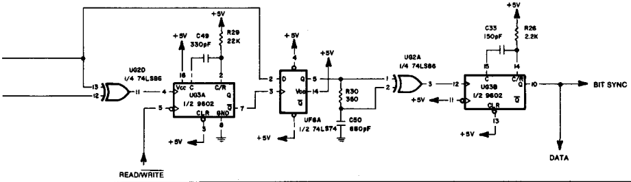
circuit, Model 1540.
